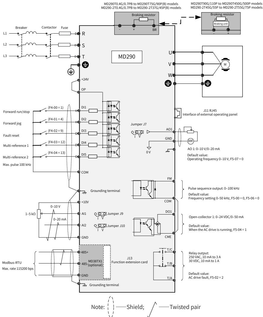
Figure 3-8 Typical wiring
