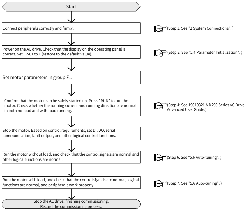
Figure 5-1 Quick commissioning
