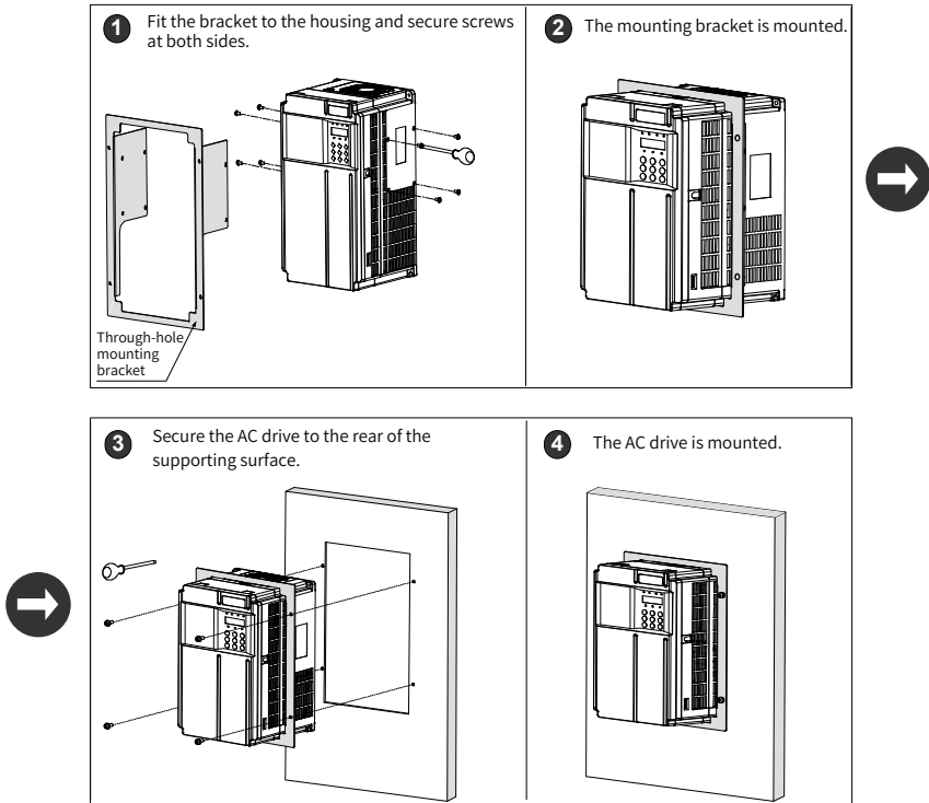
Figure 3-4 Through-hole mounting of MD290T0.4G/0.7PB to MD290T37G/45P(B) and MD290-2T0.4G/0.7PB to MD290-2T18.5G /22P(B)
