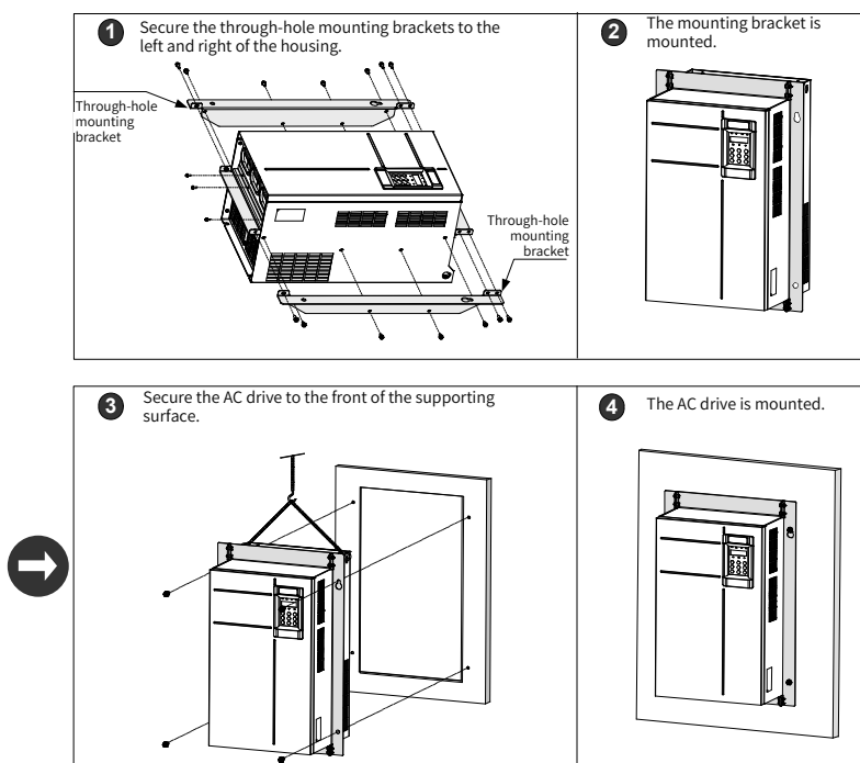
Figure 3-5 Through-hole mounting of MD290T45G/55P(B) to MD290T160G/200P and MD290-2T22G/30P(B) to MD290-2T55G/75P
