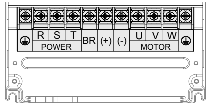
Figure 3-10 Terminal arrangement in MD290T18.5G/22P(B) to MD290T160G/200P and MD290-2T11G/15P(B) to MD290-2T55G/75P
