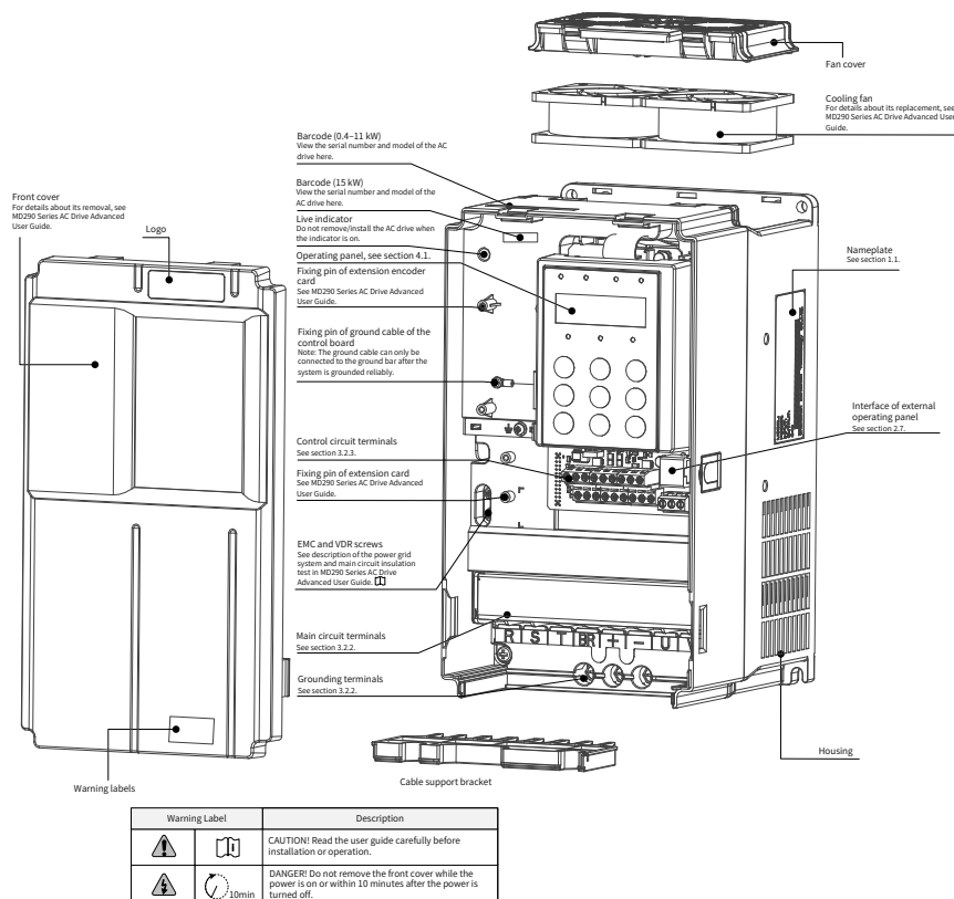
Figure 1-2 Components (MD290T0.4G/0.7PB to MD290T15G/18.5PB, MD290-2T0.4G/0.7PB to MD290-2T7.5G/11PB)
