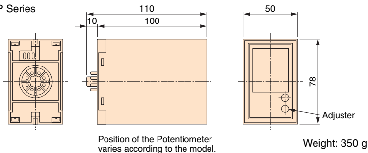
View of Socket Mounting
