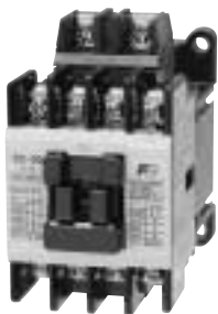
Magnetic Contactor
