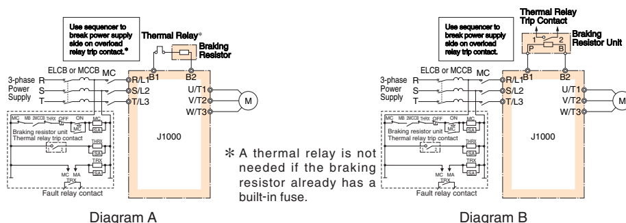
Braking Resistor [ERF-150WJ series]
