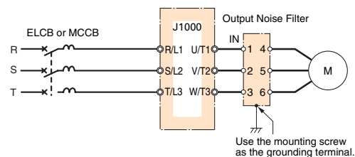
Connection Diagram
