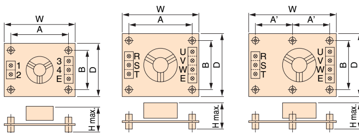
Figure 1 (Single-Phase)
