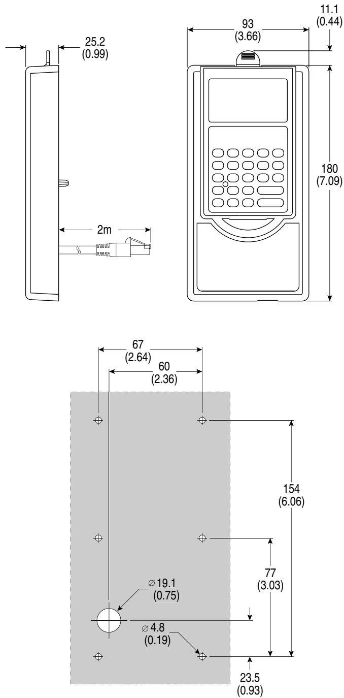
Figure B.10 NEMA Type 1 Bezel – Dimensions are in millimeters and (inches) Catalog Number: 22-HIM-B1
