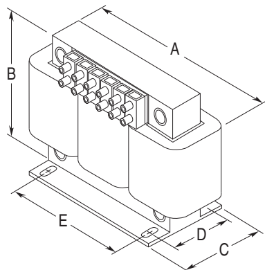
Figure B.4 Bulletin 1321-3R Series Line Reactors
