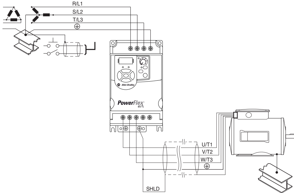
Figure 1.3 Typical Grounding
