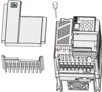
MD310T0.4 B to MD310T2.2B
