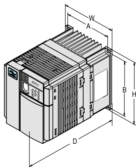
Figure 1..Model of 0.4 to 2.2 kW
