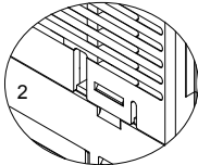
Figure 2-1 EMC jumper position and cutting method of MD310T0.4B to MD310T5.5B
