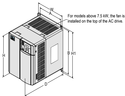
Figure 2..Model of 3.7 to 18.5 kW
