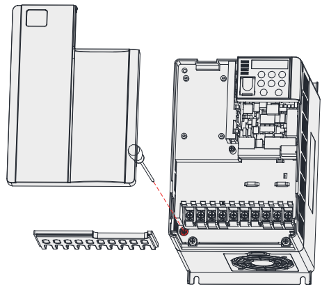
MD310T3.7B and MD310T5.5B
